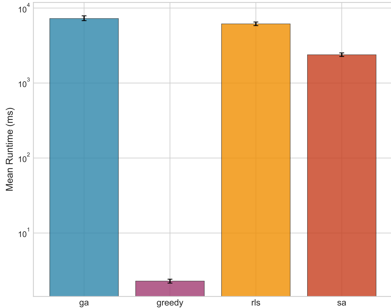
E4: Algorithm Comparison — Runtime (log scale)
