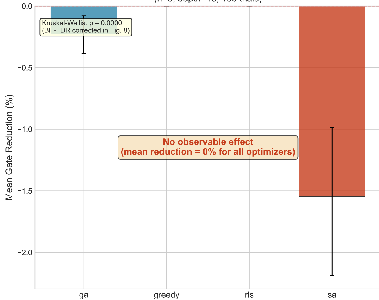
E4: Algorithm Comparison — Mean Reduction (n=5, depth=15, 100 trials)
