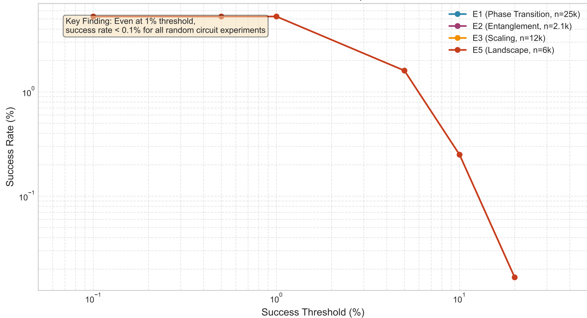
Threshold Sensitivity: Success Rate vs Threshold Across All Random Circuit Experiments
