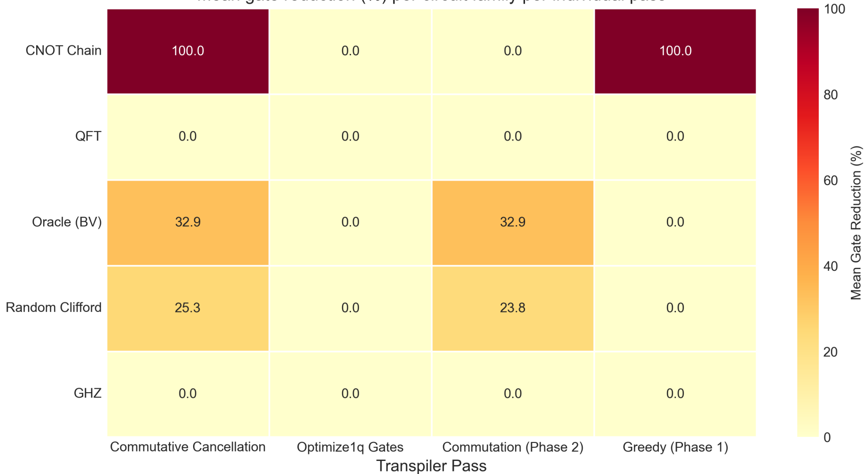
Figure 16: Pass Effectiveness Heatmap Mean gate reduction (%) per circuit family per individual pass
