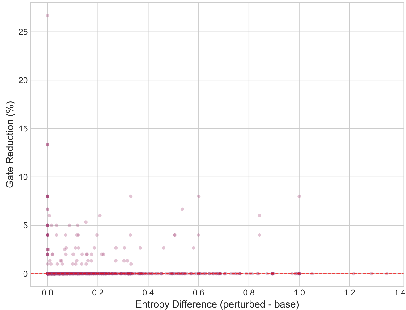
E5: Reduction vs Perturbation Magnitude (2000 sample points)
