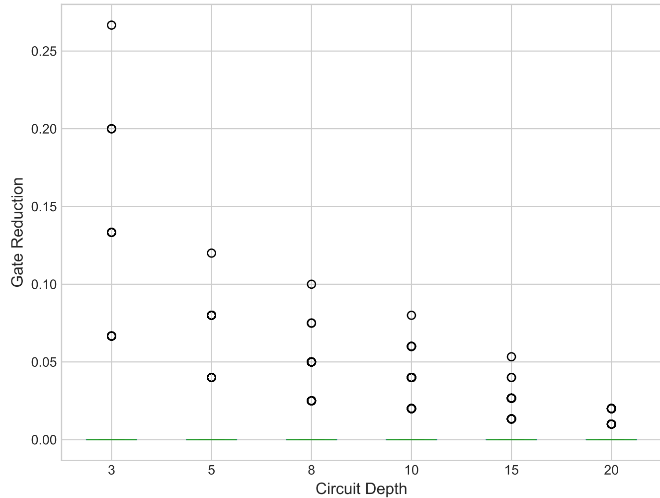
E5: Reduction Distribution by Depth
