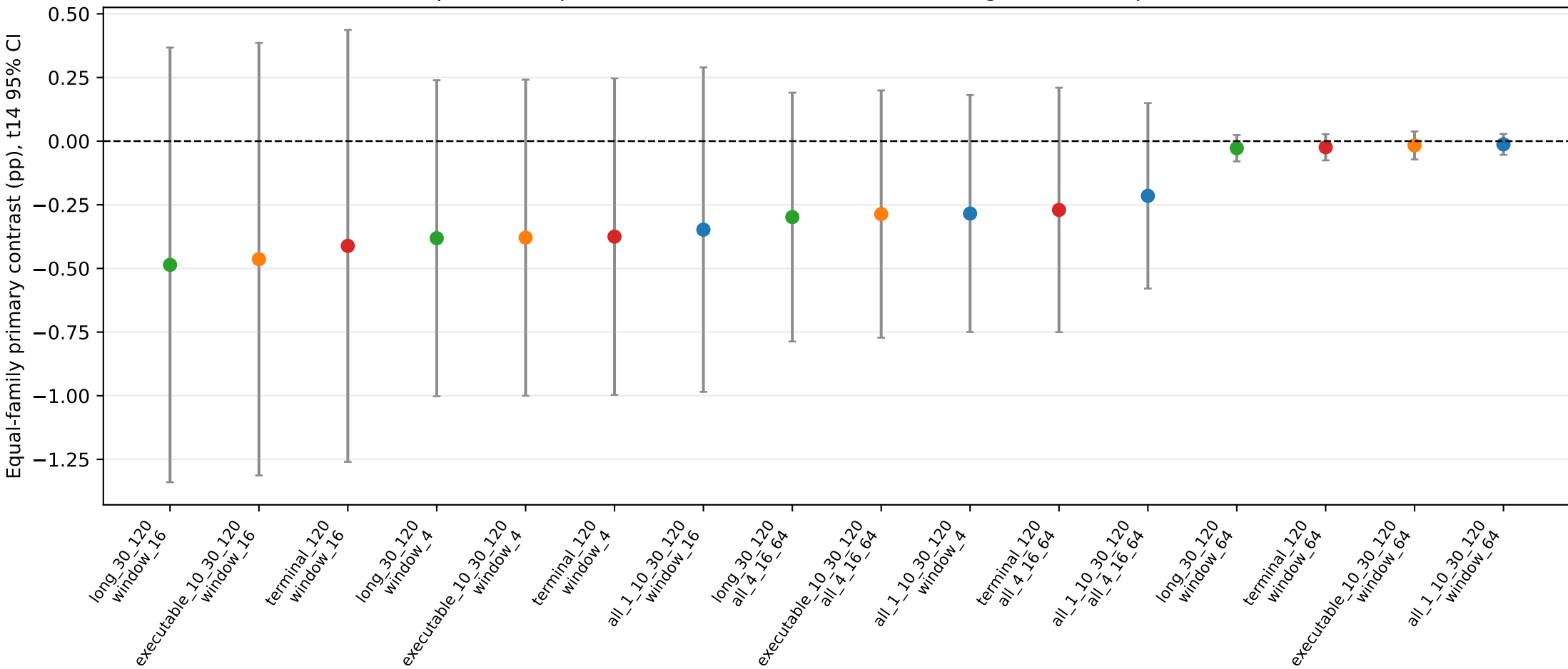
E31 post-seal specification curve (16 defensible budget/window specifications)
