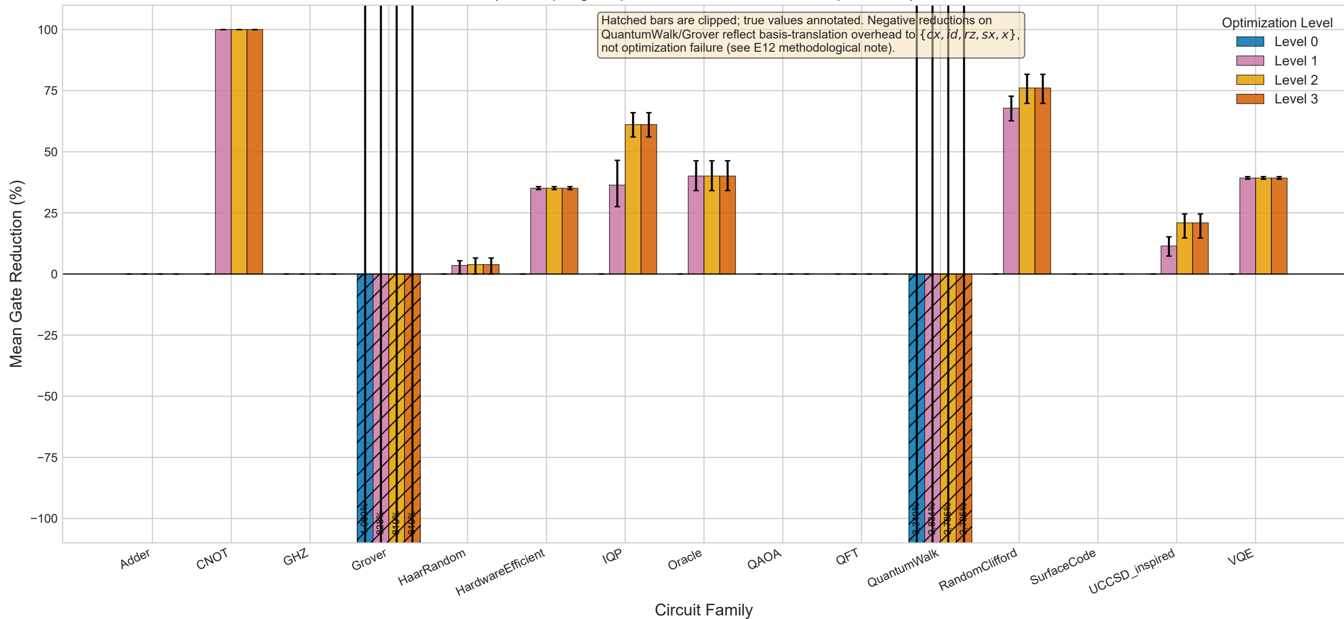
E12: Qiskit Optimization Levels vs Circuit Family (no-coupling-map mode; mean with bootstrap 95% CI)
