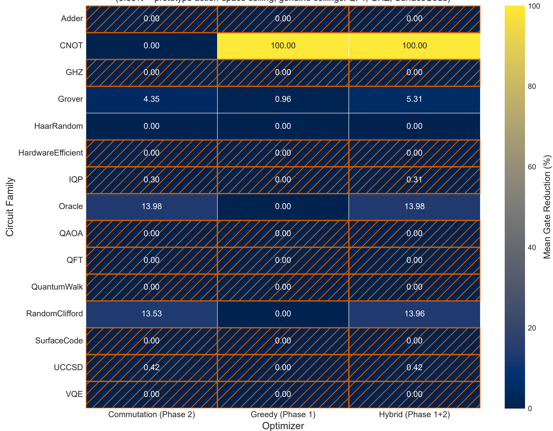
E14: Extended Benchmark - Mean Gate Reduction (%) 15 Circuit Families x 3 Optimizers (0.00% = prototype action-space ceiling; genuine ceilings: QFT, GHZ, SurfaceCode)
