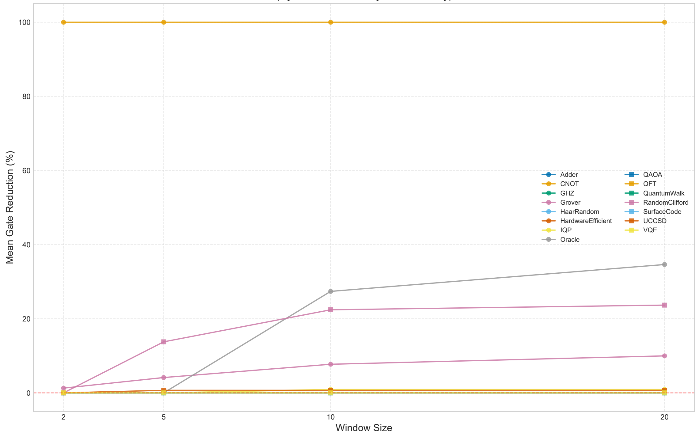
E16: Window Scaling — Reduction Saturation Curves (Hybrid Phase 1+2, by Circuit Family)
