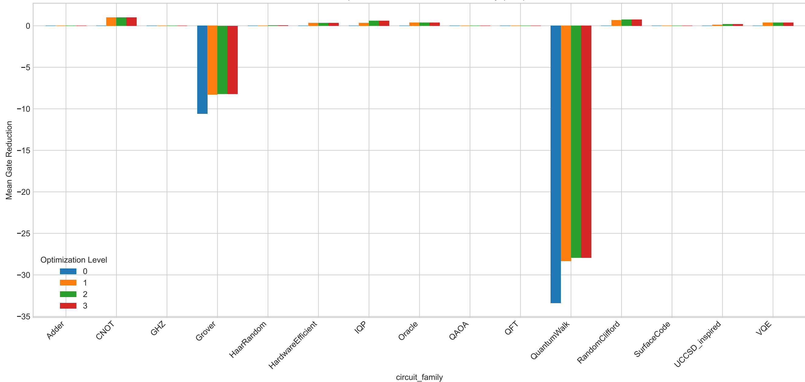
Qiskit Optimization Levels vs Circuit Family (E12)
