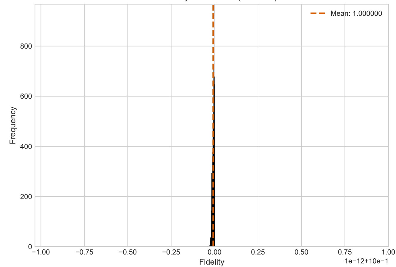
E3: Fidelity Distribution (n=11962)
