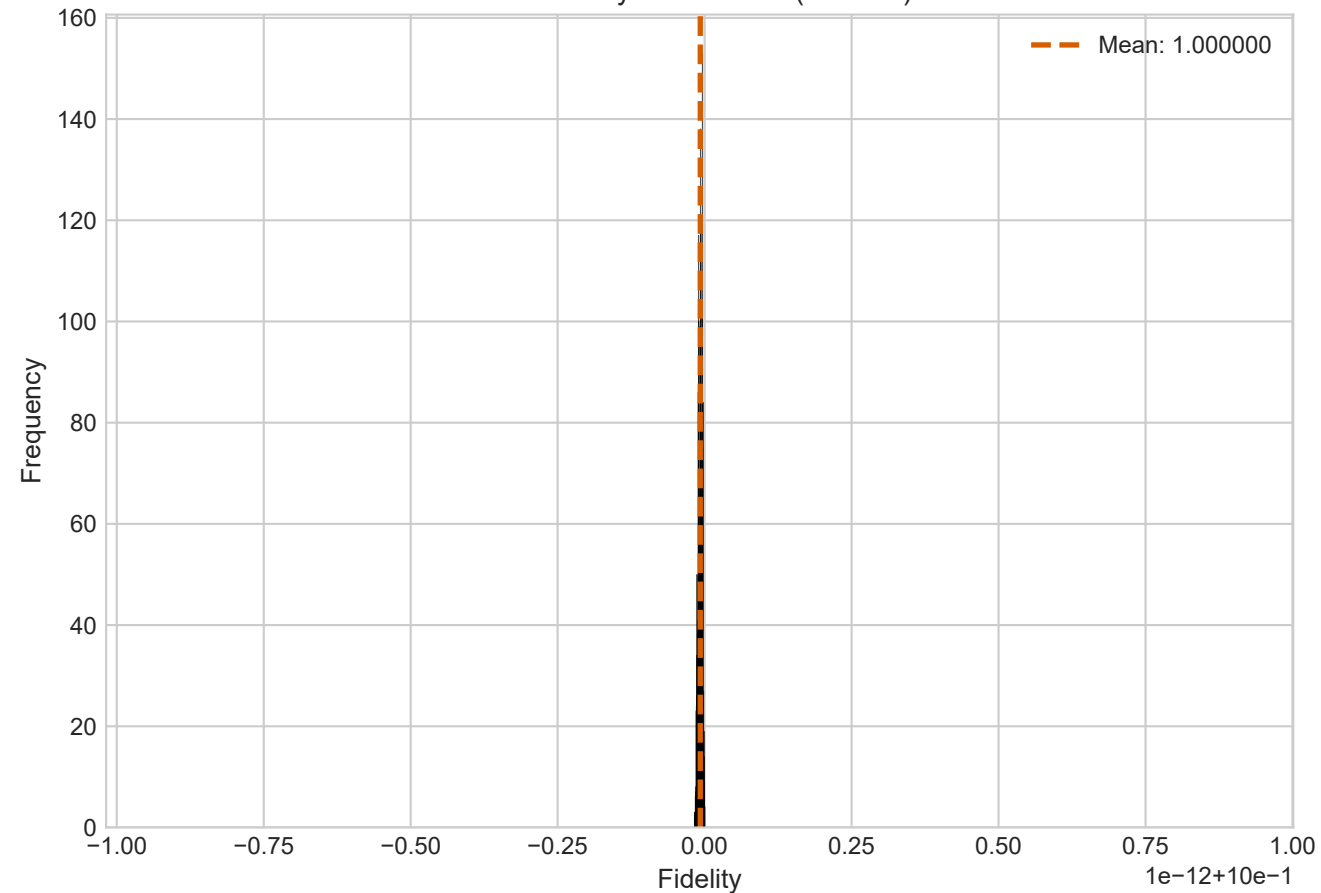
E5: Fidelity Distribution (n=6000)
