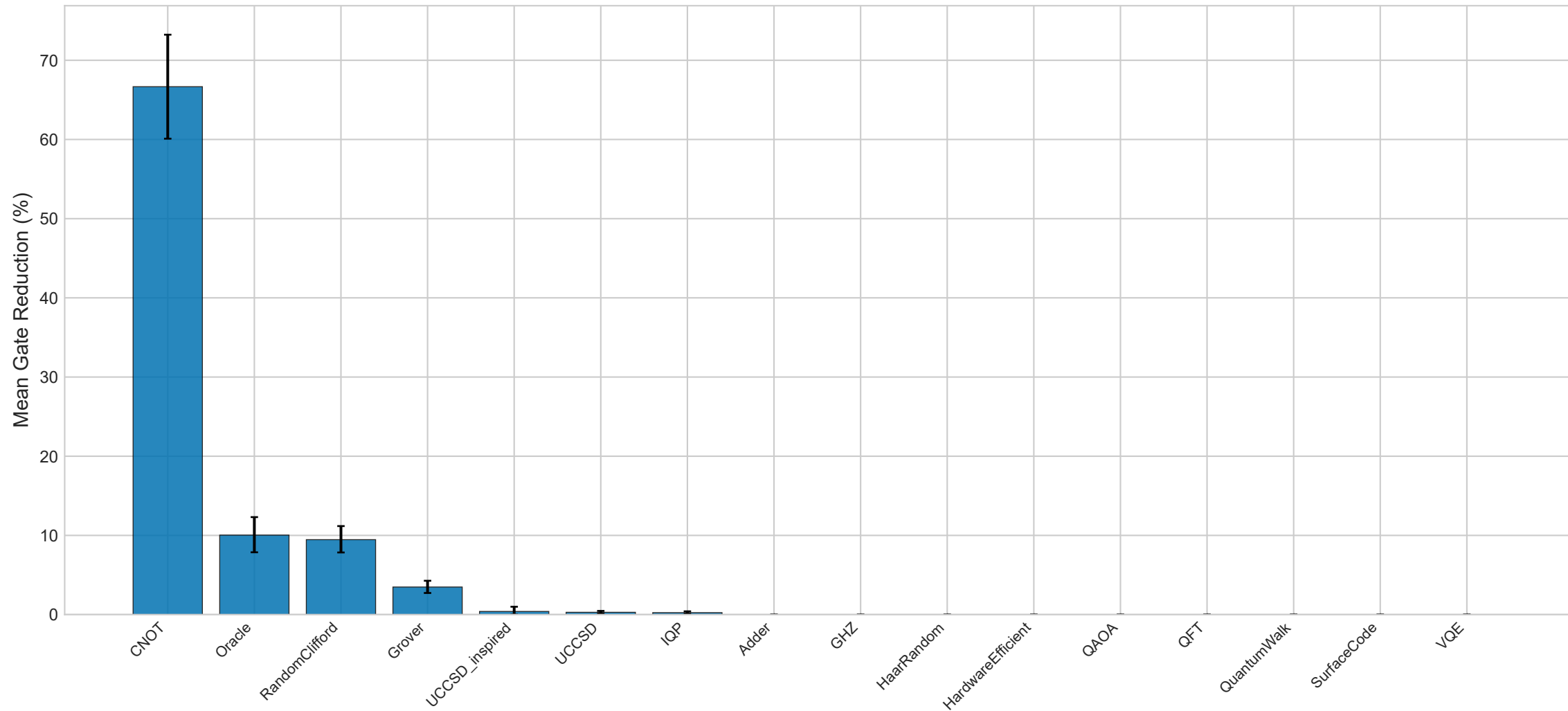
Real-Circuit Optimizer Comparison (E11/E14) (mean gate reduction per family, bootstrap 95% CI)
