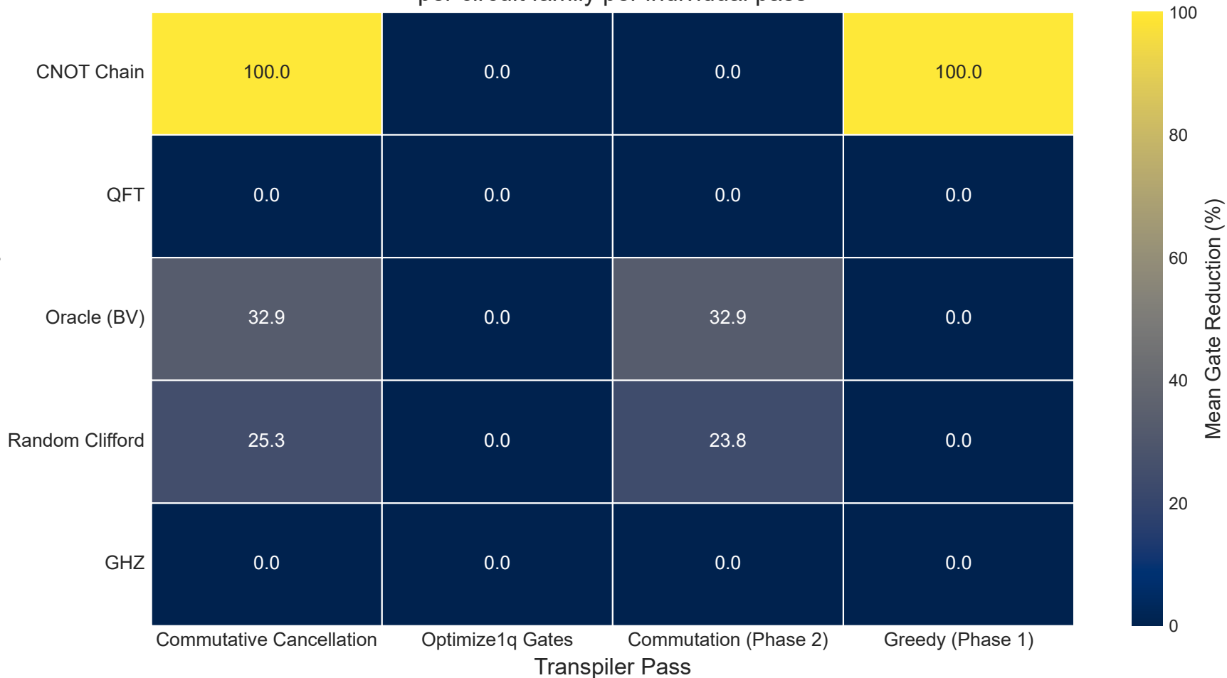
Pass Effectiveness Heatmap — Mean Gate Reduction (%) per circuit family per individual pass
