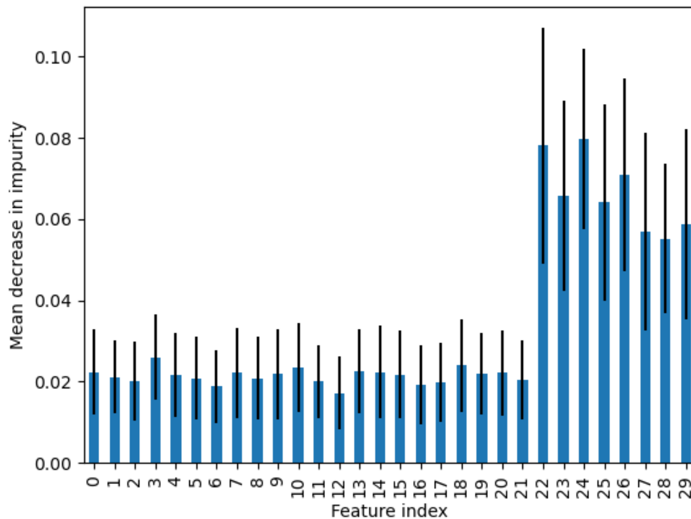
Feature importances using mean decrease in impurity
