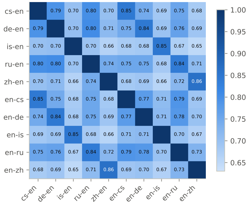
FLAP gen 40%: FFN channel Jaccard
