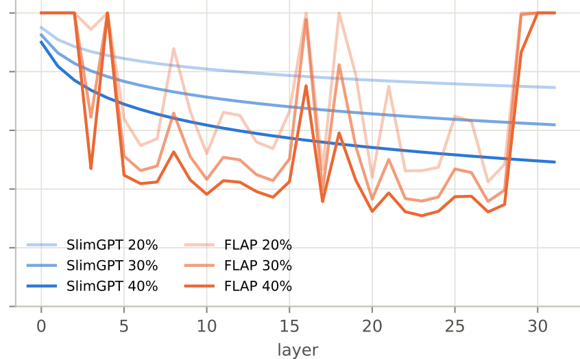
FFN channels kept
