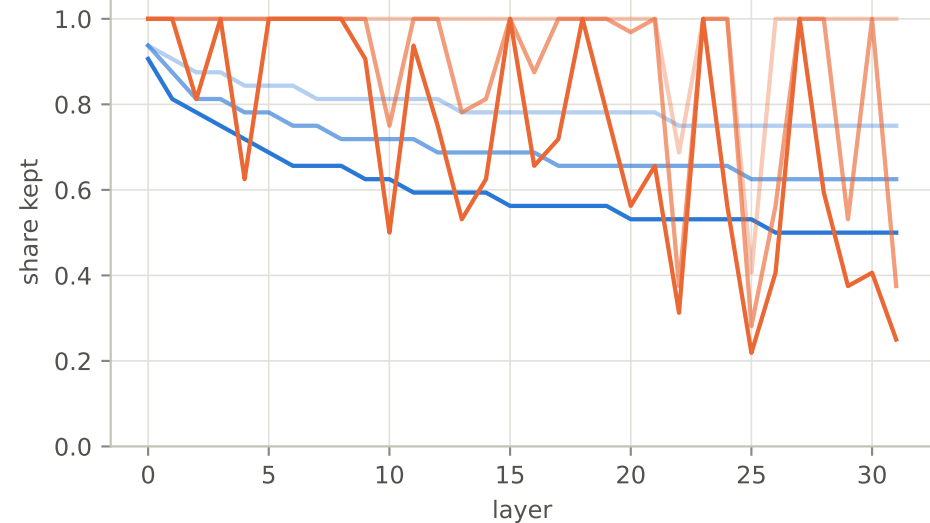
attention heads kept
