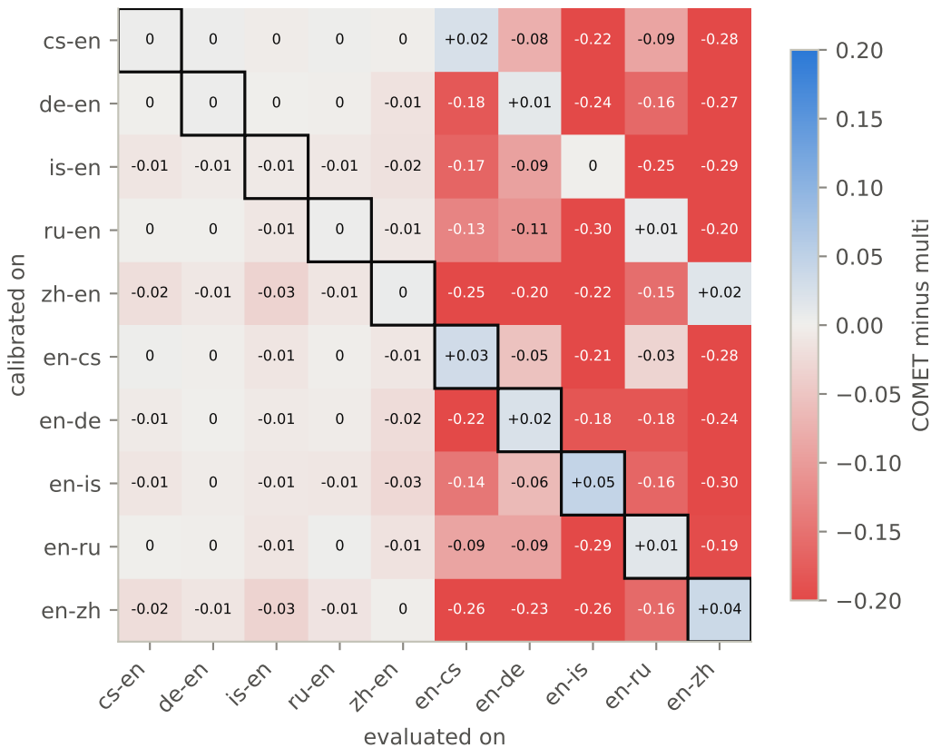
SlimGPT gen 40%: COMET minus multi, full test sets
