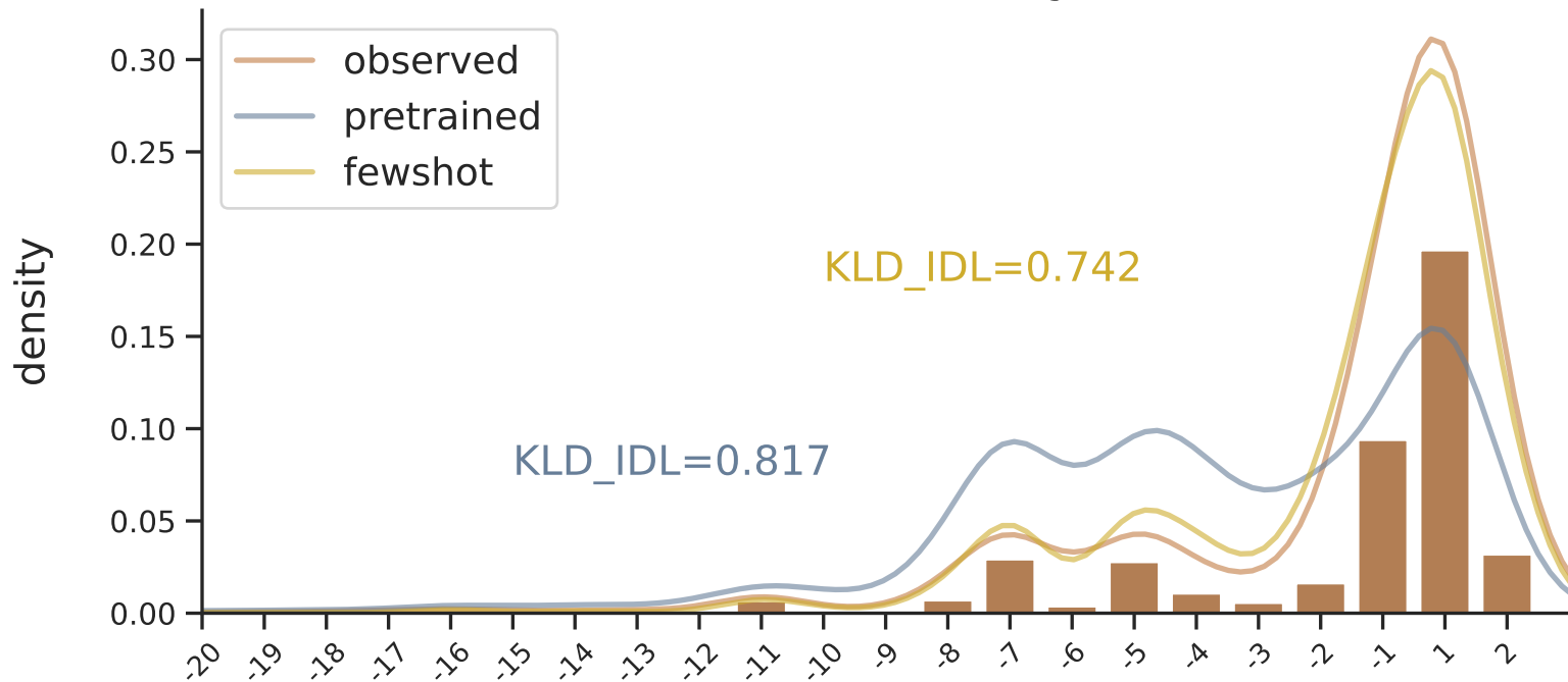
Overall distribution of Indel length (mESC)
