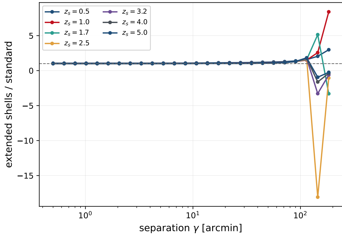
cost of the \lambda_{\min} floor
