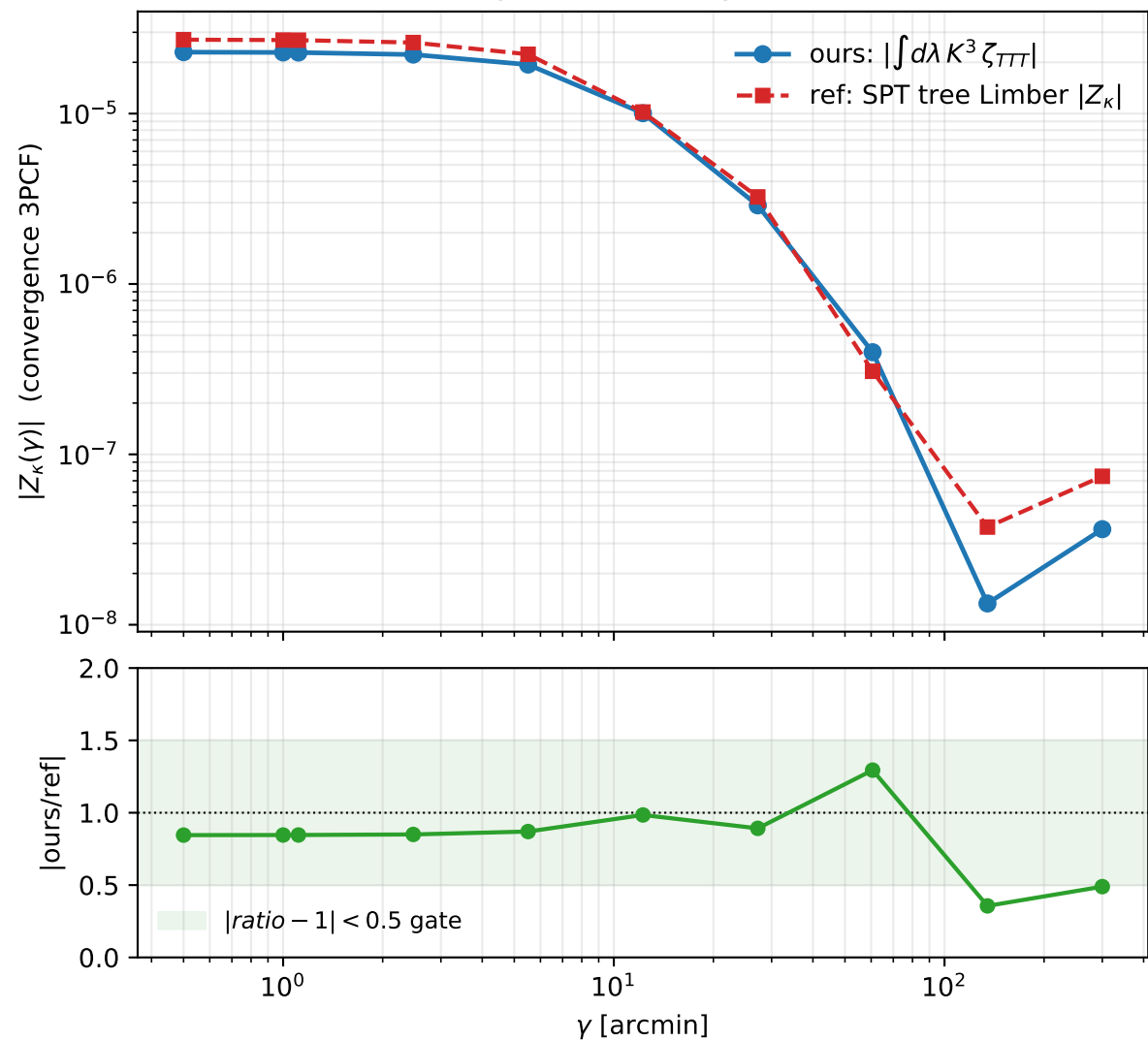
STAGE 0: scalar convergence 3PCF, squeezed, z_s = 5 (both Z_\kappa < 0 )
