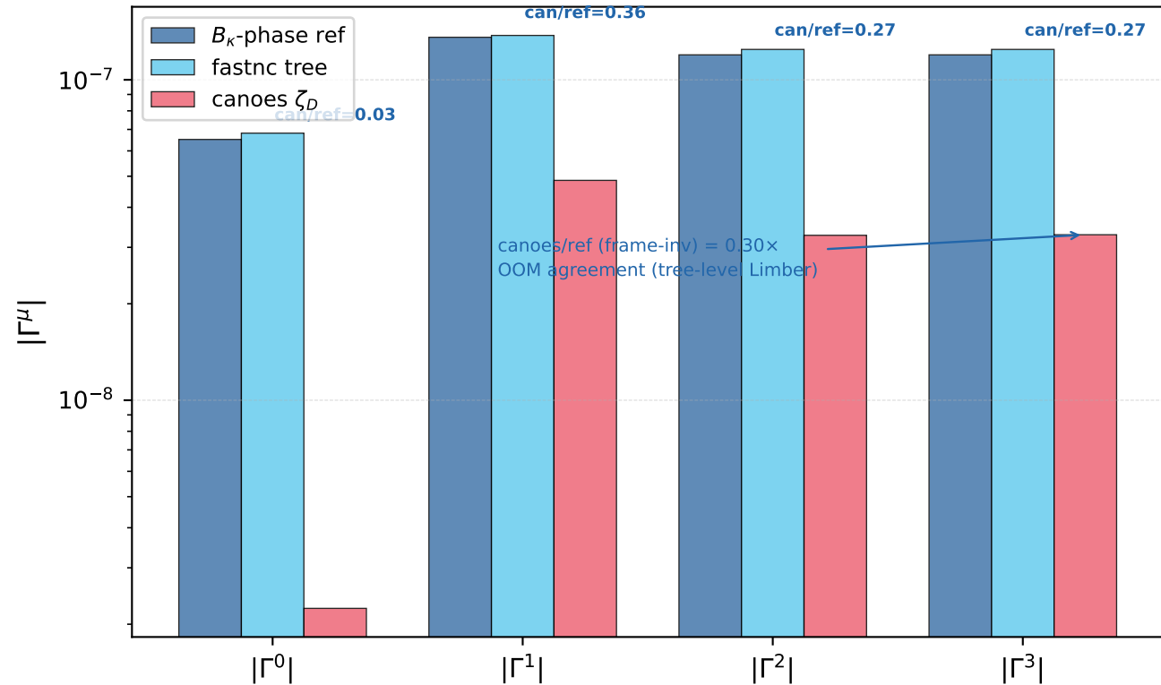
Per-component |\Gamma^\mu| at primary point ( \gamma = 10' , \phi = 60^\circ , z_s = 5 )
