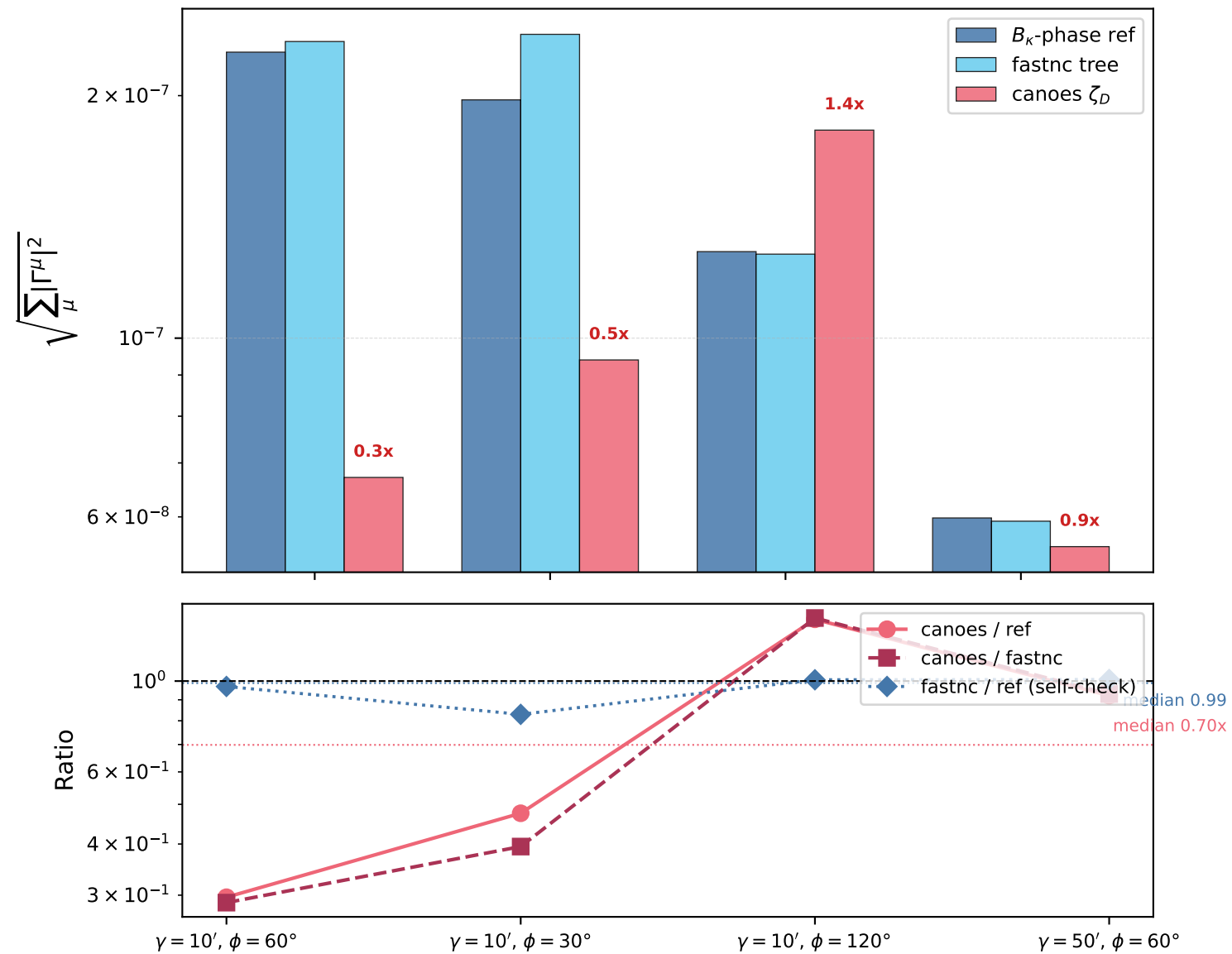
Three-way frame-invariant shear 3PCF: B_K -phase ref vs fastnc vs canoes \zeta_D
