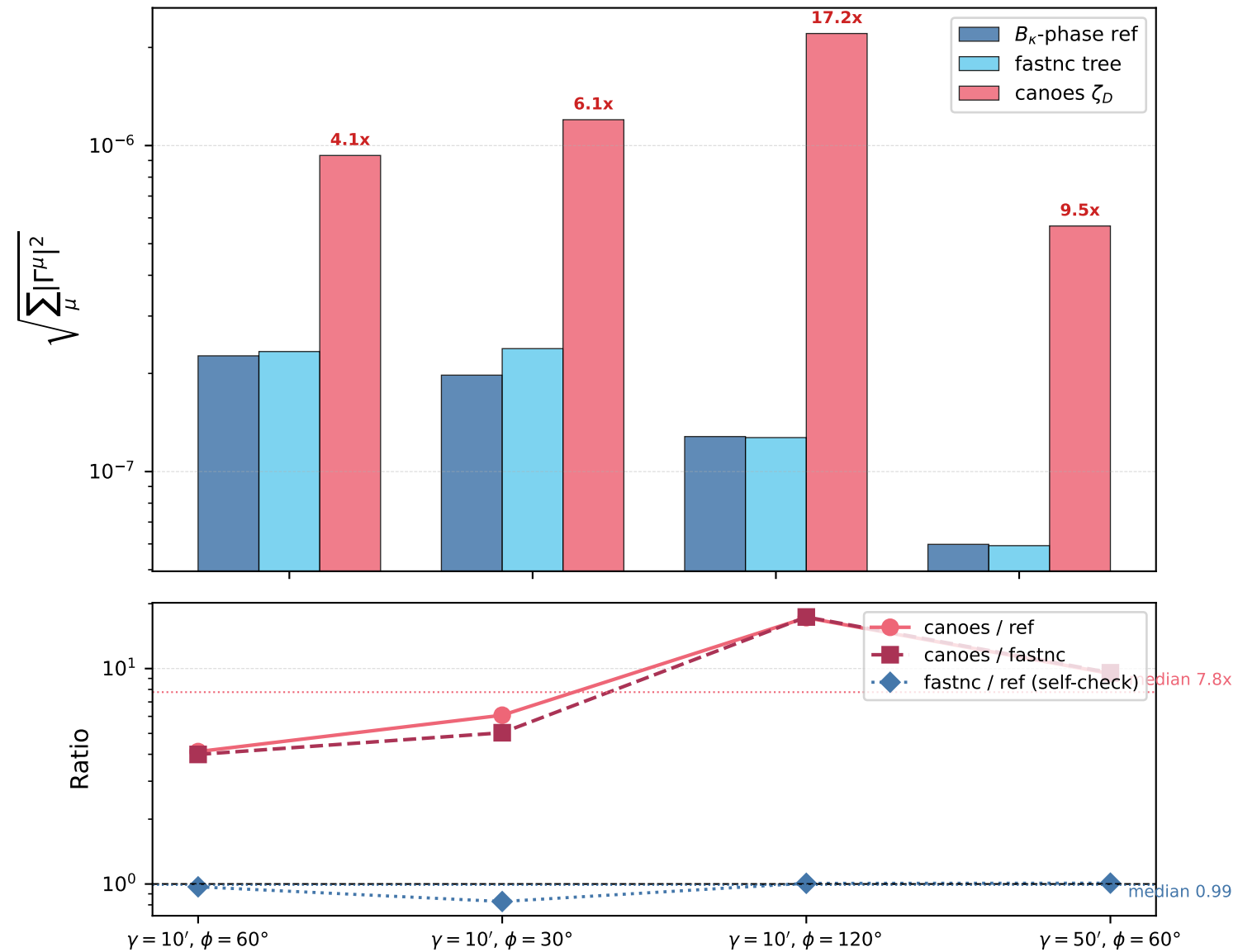
Three-way frame-invariant shear 3PCF: B_\kappa -phase ref vs fastnc vs canoes \zeta_D
