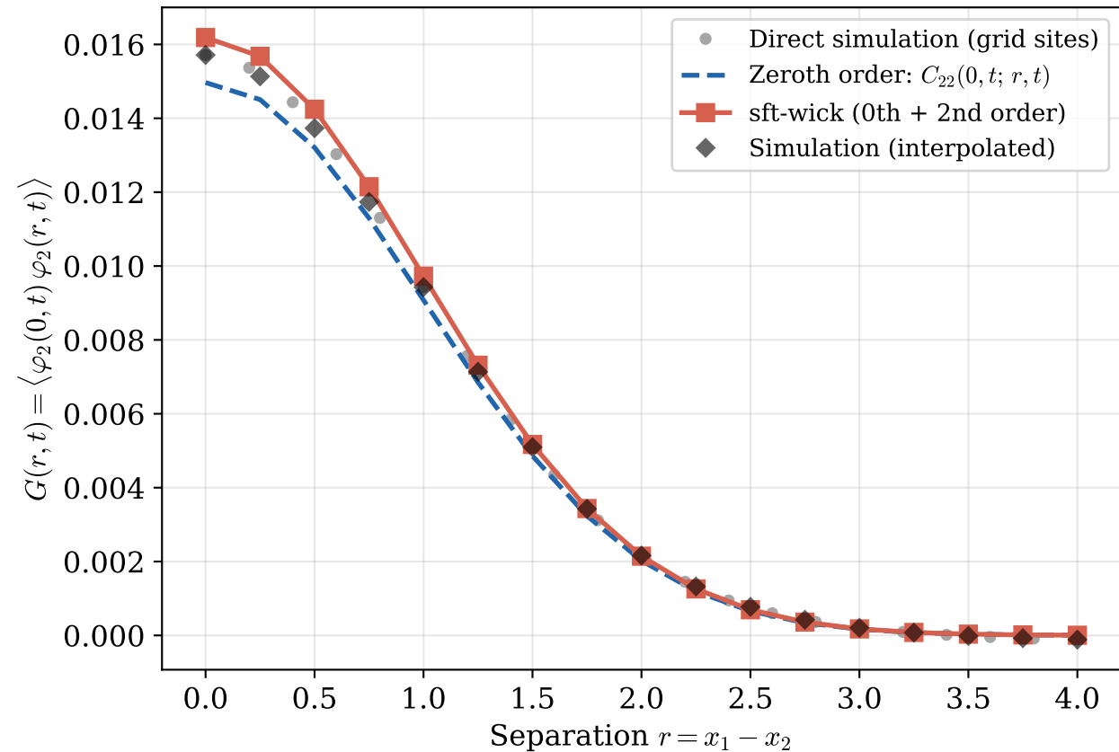
Two-point correlator \langle \varphi_2 \varphi_2 \rangle at t = 3.0
