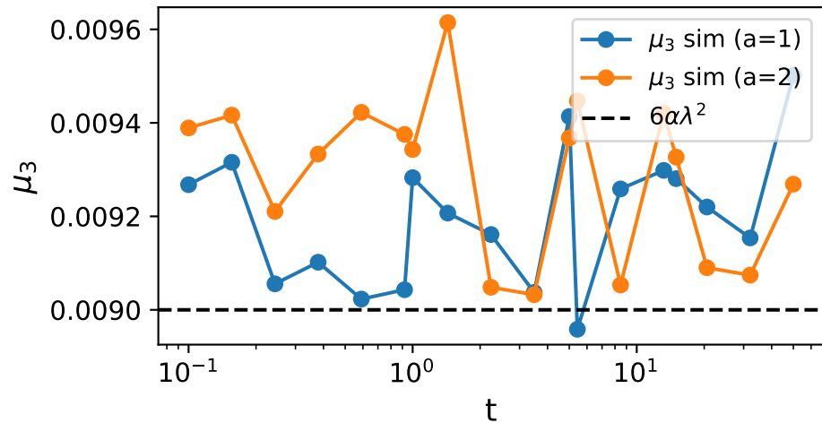
3rd moment of \tilde{\eta}_a(0, t)
