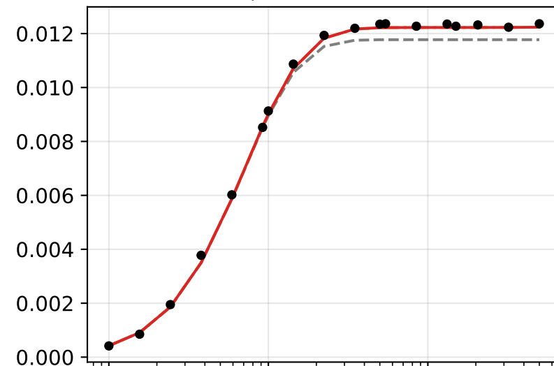
\xi_{11}(r=0.0, t)
