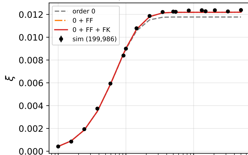
\xi_{00}(r=0.0, t)
