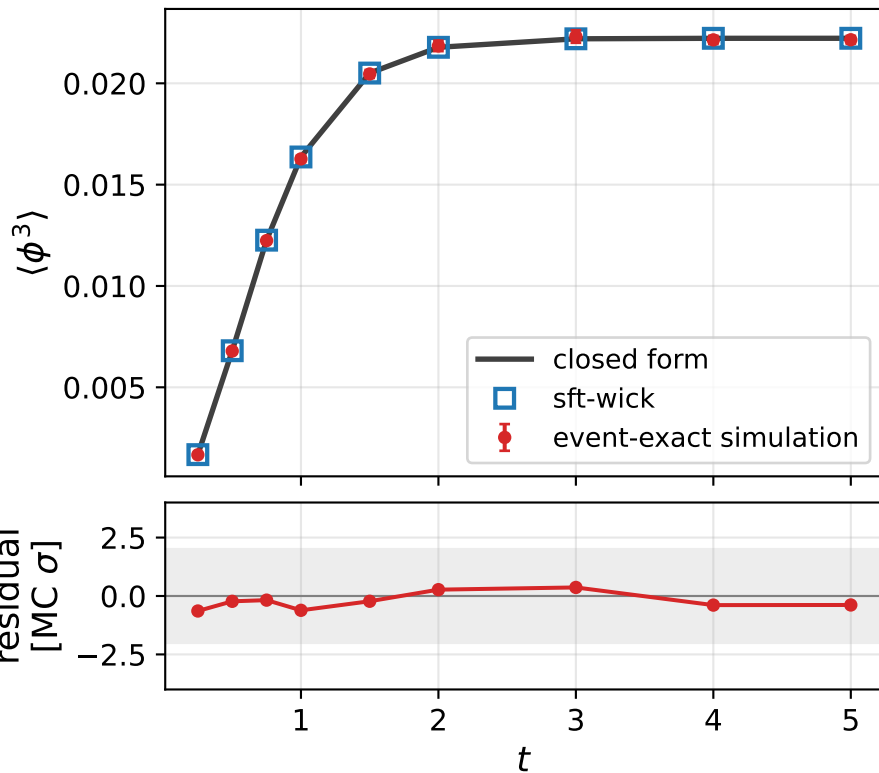
\langle \phi(0, t)^3 \rangle (all points coincident)
