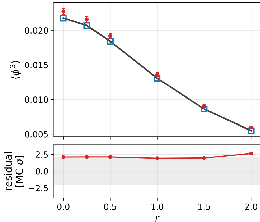
\langle \phi(0, t)^2 \phi(r, t) \rangle , t = 2
