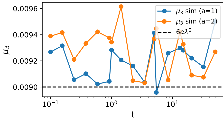
3rd moment of \tilde{\eta}_a(0, t)
