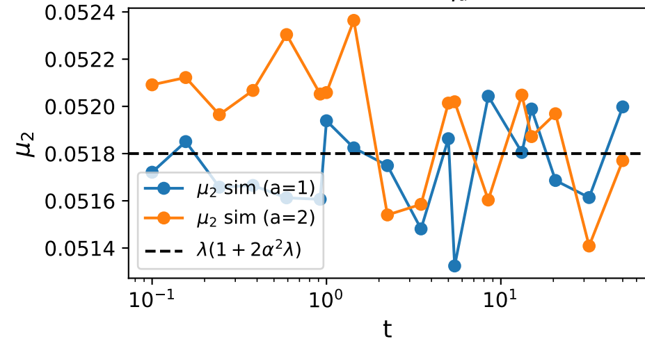
2nd moment of \tilde{\eta}_a(0, t)
