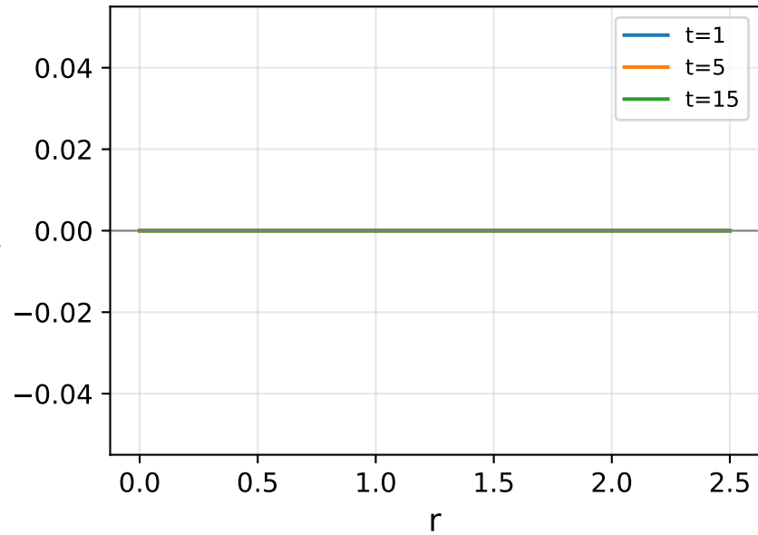
FK contribution to \xi_{00}
