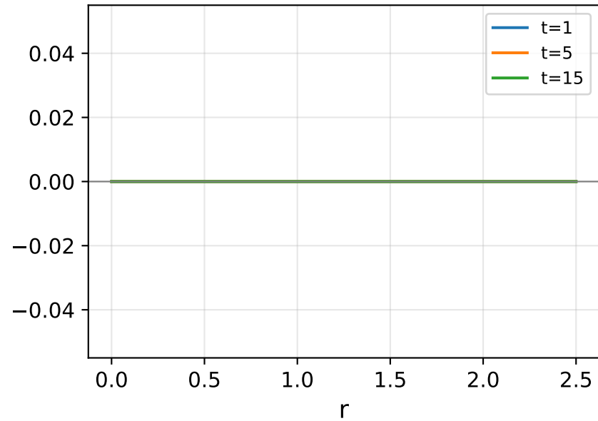
FK contribution to \xi_{11}
