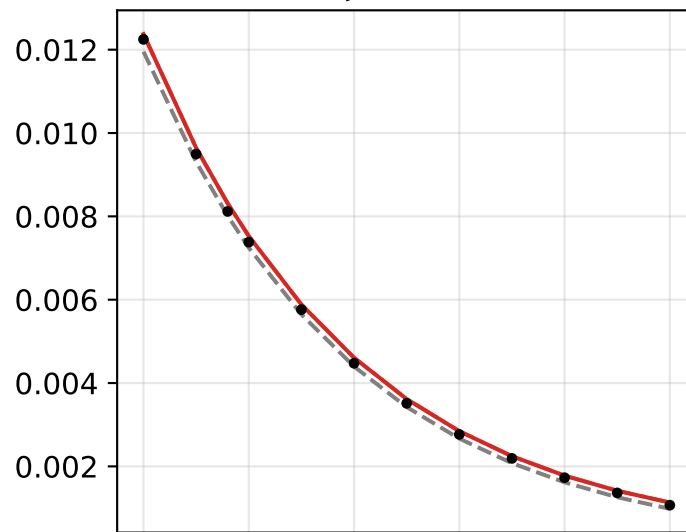
Demo 2 \xi_{ab}(r) at selected t ( \alpha = 0.6 )
