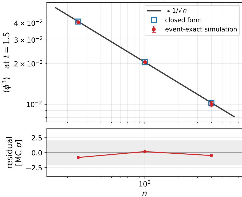
Non-Gaussianity knob n = \nu \sigma_t \sigma_x ( \kappa_2 held fixed by compensating h )
