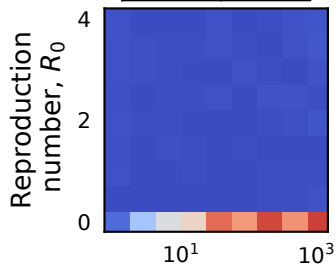
g_{0,N \rightarrow N^*} g_{0,E \rightarrow 2E} 0.0 0.5
