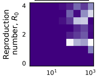
\psi_{Ag} -1 0 1
