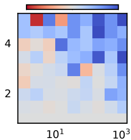
g_{0,N \rightarrow N^*} = g_{0,E \rightarrow 2E}
