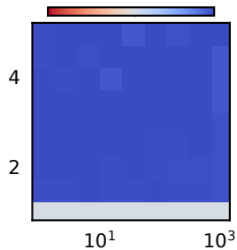
g_{0,N \rightarrow N^*} = g_{0,E \rightarrow 2E}
