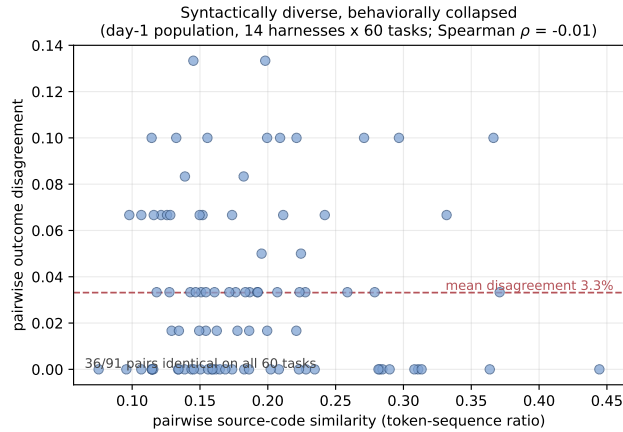
Figure 3: Syntactic diversity vs. behavioral collapse (Phase I, discovery; day-1 population: 14 harnesses \times 60 tasks, 91 pairs including the bare and react baselines). Each point is a harness pair; x = token-sequence code similarity, y = fraction of tasks with differing correctness. Code similarity does not predict outcome disagreement ( \rho = -0.01 ); 36/91 pairs are identical on all 60 tasks. Raw pairs: fig1.phenomenon_data.json in the code release.
