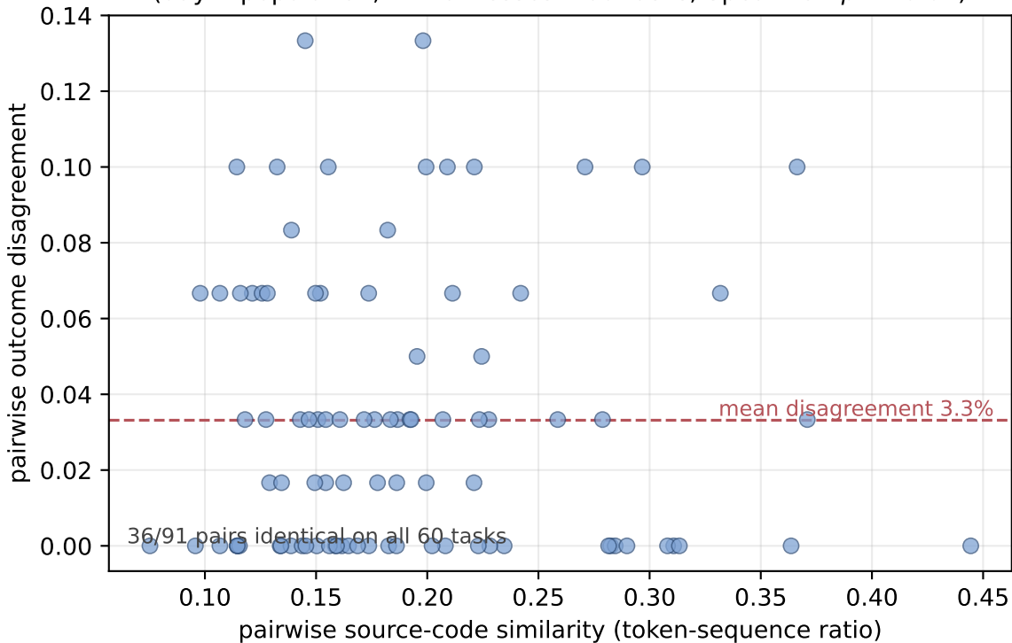
Syntactically diverse, behaviorally collapsed (day-1 population, 14 harnesses x 60 tasks; Spearman \rho = -0.01 )
