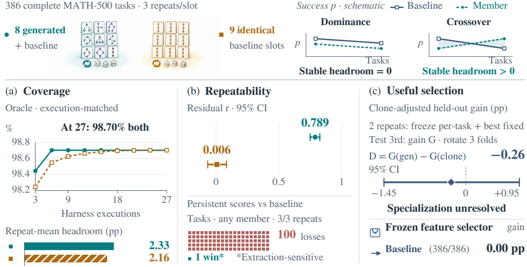
Figure 1: Coverage, repeatable scores, and useful selection on 386 complete MATH tasks. Both arms freeze per-task choices and a best fixed member on two repeats, then measure gain G on the held-out repeat. D subtracts the same-code gain. Oracle budgets count harness executions. Intervals are 95% bootstrap CIs; the sole persistent win is extraction-sensitive. The top-right sketches are population success-probability examples, not observed task curves. Stable complementarity requires the better member to change across tasks.
