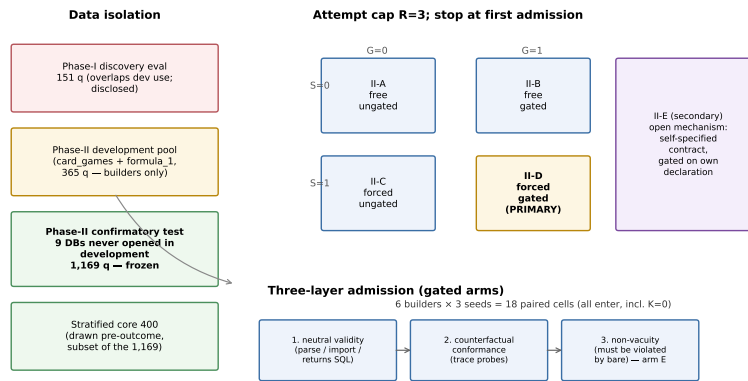
Phase-II confirmatory design: database-level isolation, 2 \times 2 factorial + open-mechanism arm, three-layer admission
