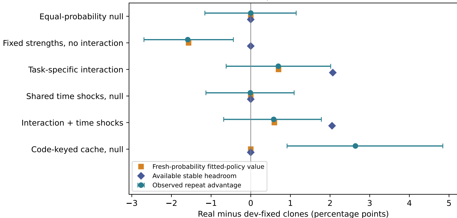
200 tasks, 4 repeats: different estimands
