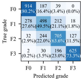
(a) Confusion, Baseline (A)
