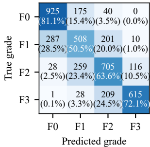
(b) Confusion, SynAP-Fib (E)
