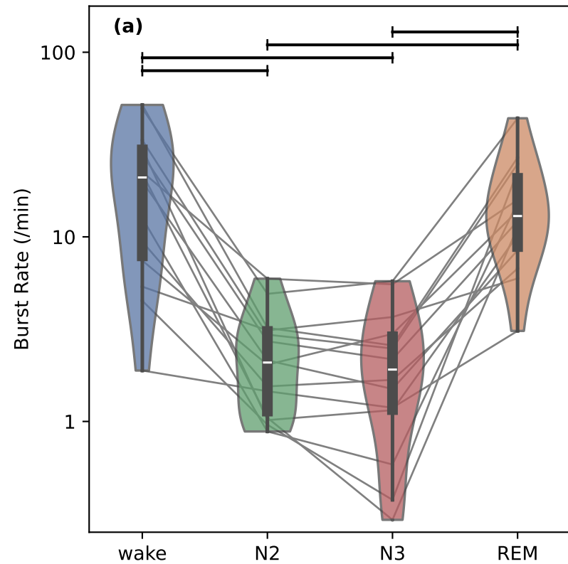
Wake- and REM- Specific Oscillation
