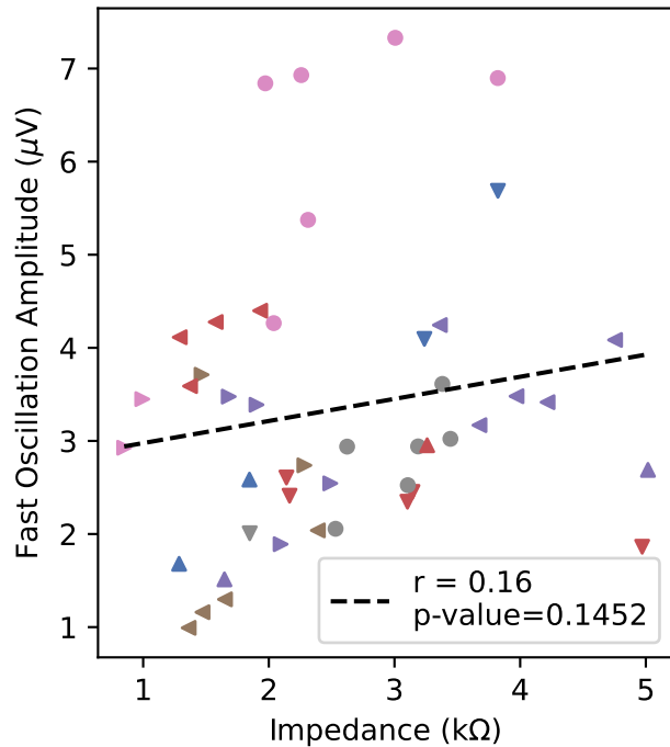
(c) Fast Oscillations
