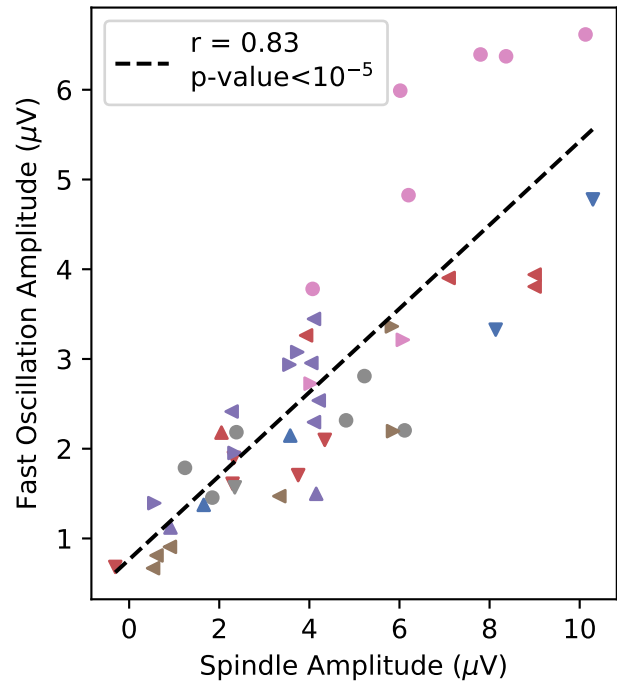
(a) Amplitudes after regressing out impedance
