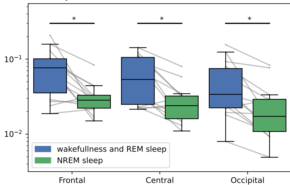
(C) Mean wPLI for Fast Oscillations
