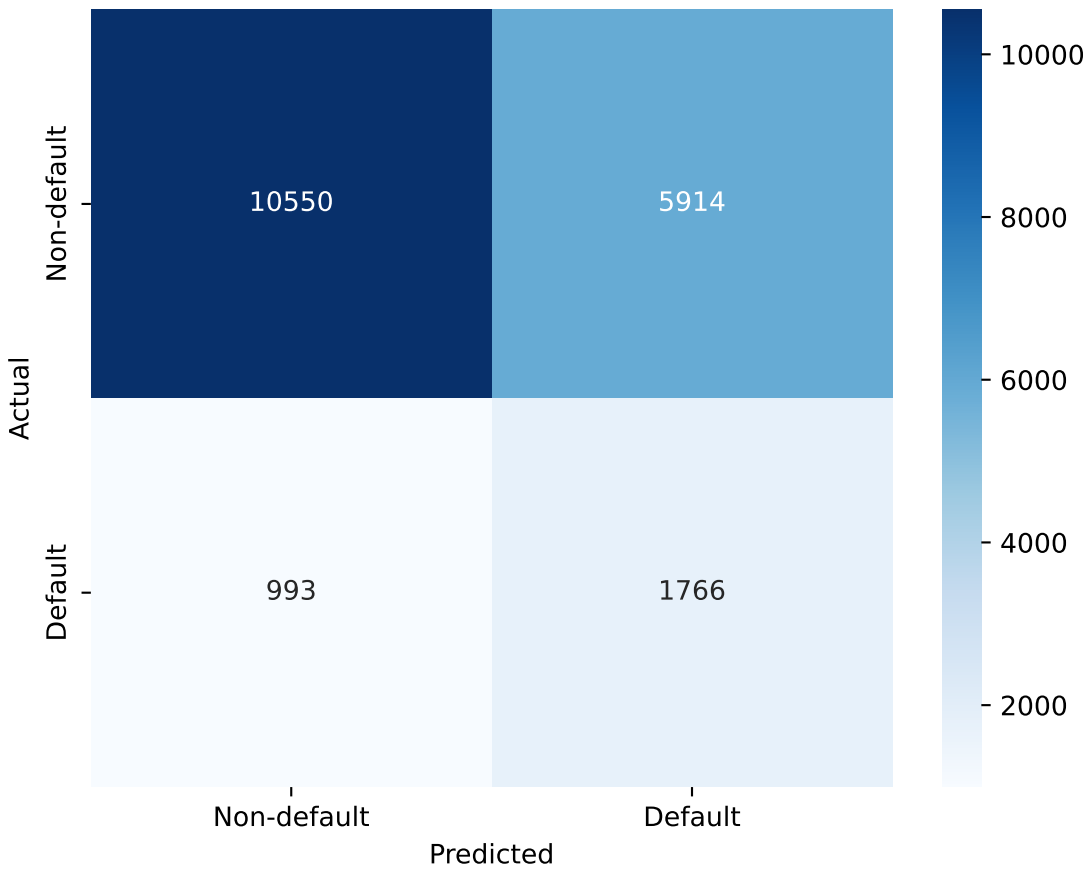
Confusion Matrix: Final Model
