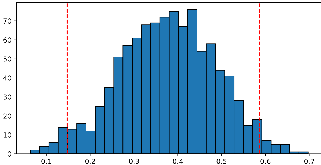
Bootstrap Distribution of Average Tau
