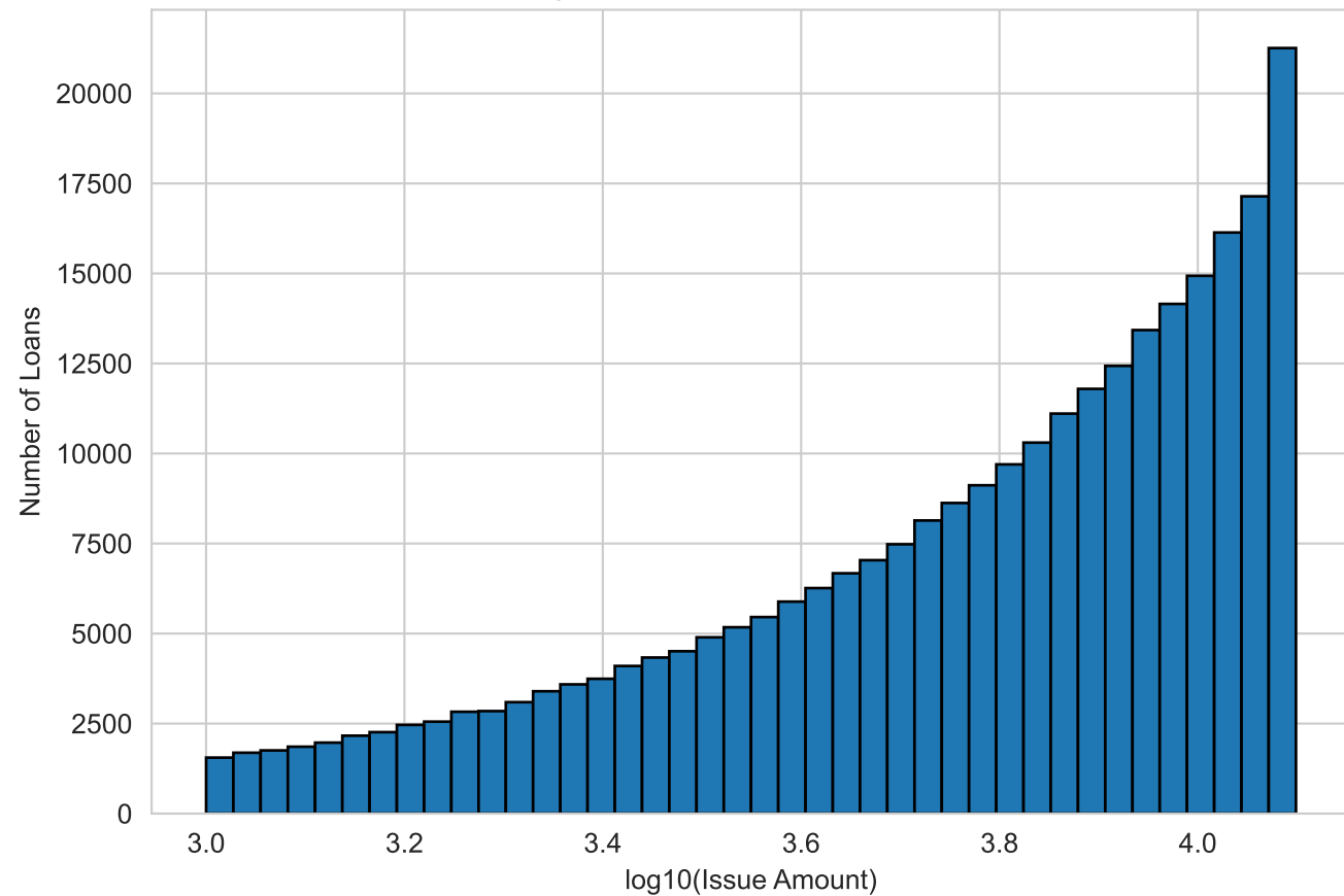
Log Distribution of Issue Amount
