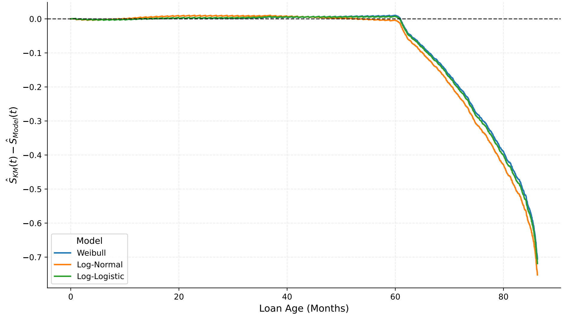
Parametric Survival Fit Error Relative to Kaplan-Meier
