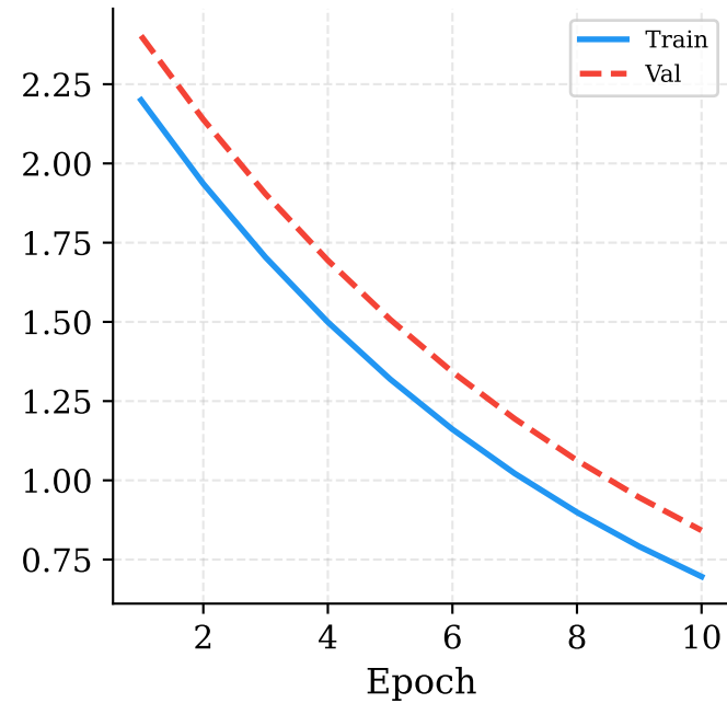
Loss Curves
