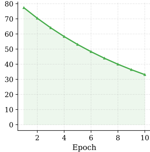
CER (%)
