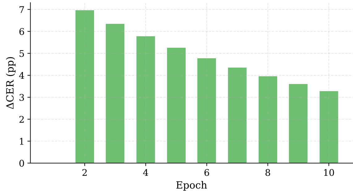
CER Improvement per Epoch
