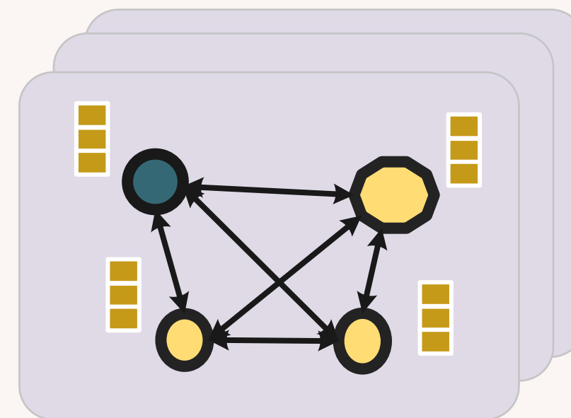
Graph Convolutional Layers
