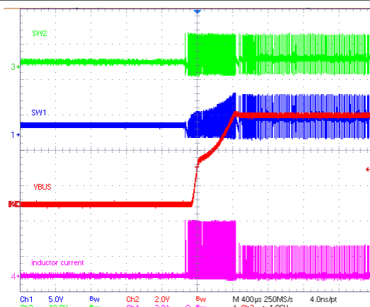
VBUS = 15V VBAT = 8V ICHG = 0A Figure 8-11. Buck Mode PFM with OOA
