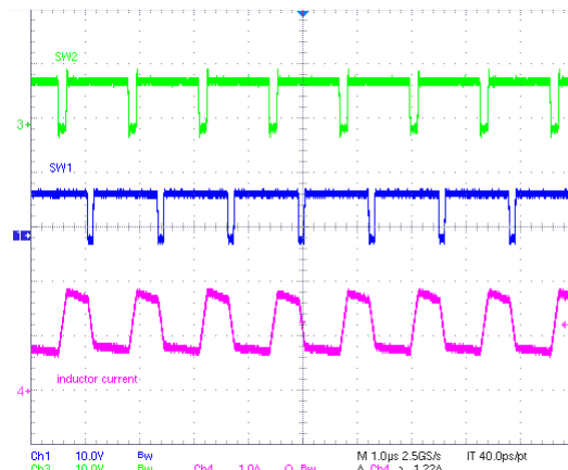
VBUS = 8V VBAT = 8V ICHG = 1A Figure 8-9. Buck-Boost Charging Mode PWM Operation
