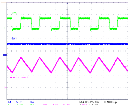
VBUS = 5V VBAT = 8V ICHG = 1A Figure 8-8. Boost Charging Mode PWM Operation
