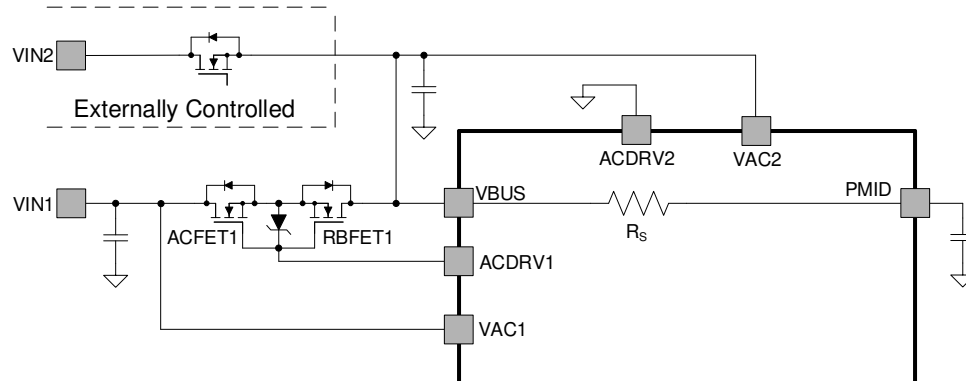
Figure 7-3. One ACFET-RBFET Structure Supporting One Input at VAC1 and/or One Input at VBUS
