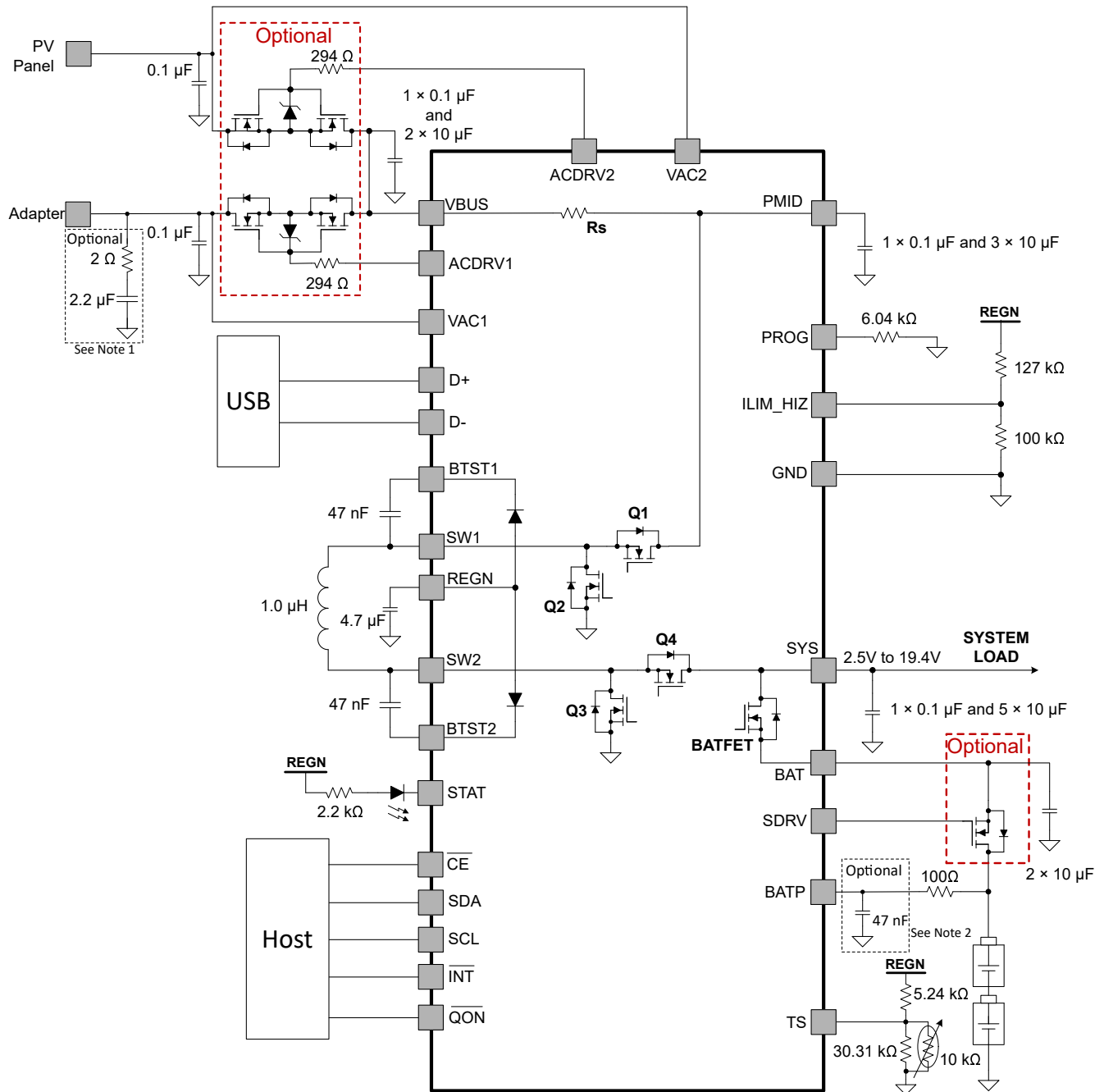
Figure 8-2. BQ25798 Application Diagram with Two Input Sources and Ship FET
