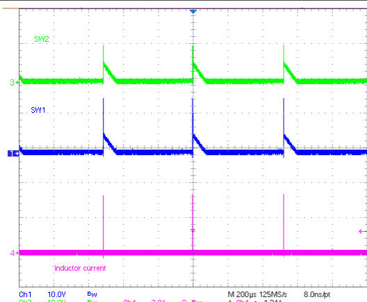
VBUS = 15V VBAT = 8V ICHG = 1.5A Figure 8-10. Buck Charging Mode PWM Operation
