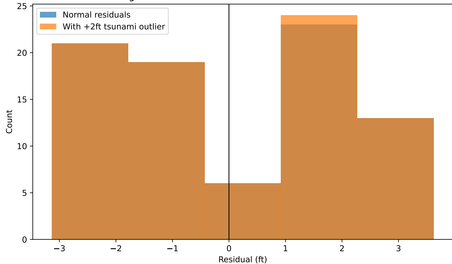
Histogram of Residuals With and Without Tsunami Outlier
