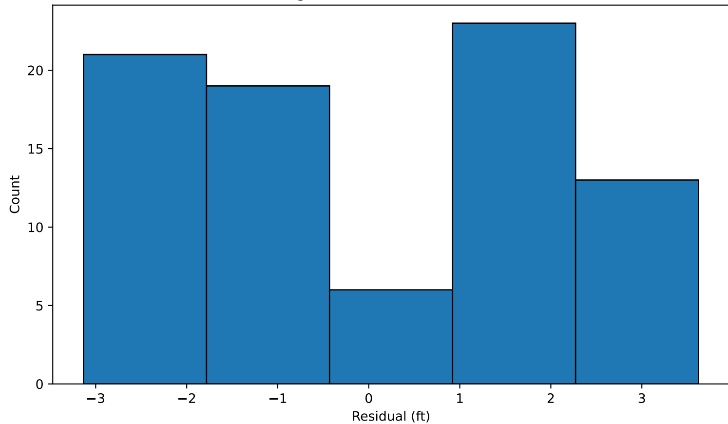
Histogram of Tide Model Residuals
